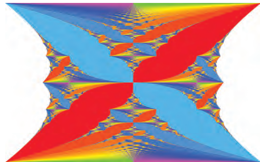
Figure 2. The colored Hofstadter butterfly.
